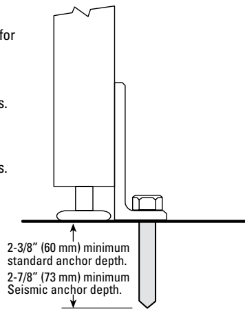
Anchorage Detail
