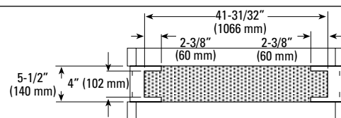
Top Access Reagent Island Cores
