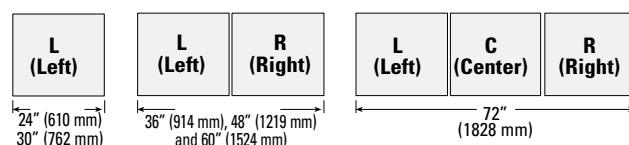
Frame Widths
