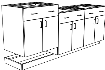
Applied Plywood Ladder Toebase
